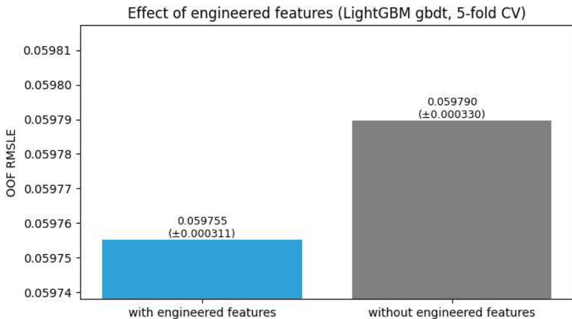
Figure 5: OOF RMSLE comparison for LightGBM (gbdt) with and without engineered features.
